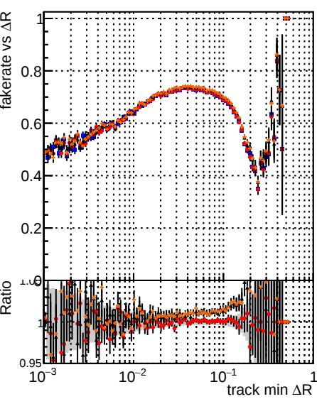
Fake rate vs \Delta R(\text{track, jet}) Legend: DOM mktFit T-Original DOM mktFit T-Improved DOM mktFit T-NEWHS-100 DOM mktFit T-NEWHS-100-improved
