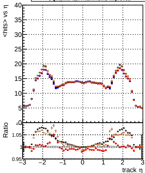
mean hit DQM_mkFit_TToriginal DQM_mkFit_TTNEWHMS-improved DQM_mkFit_TToriginal-106 DQM_mkFit_TTNEWHMSMS-improved
