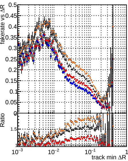
Fake rate vs \Delta R(\text{track, jet}) Legend: DOM mkeFit Original DOM mkeFit TRIMMS-improved DOM mkeFit NEWHS-improved DOM mkeFit TRIMMS-improved DOM mkeFit NEWHS-improved
