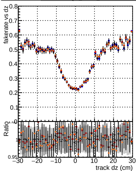
Fake rate vs dz — DGM mkt fit T Toriginal Tnew TnewHSMs-improved — DGM mkt fit T Toriginal Tnew TnewHSMs-improved
