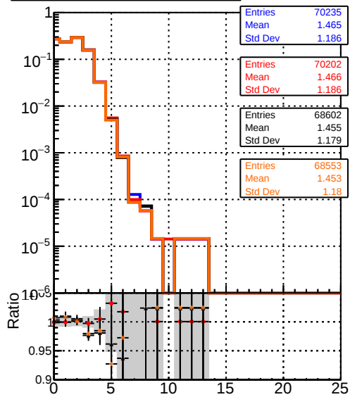
DQM_mkFit_TToriginal DQM_mkFit_TTNEWHMS-improved DQM_mkFit_TTOriginal-106 DQM_mkFit_TTNEWHMSMS-improved mean hits
