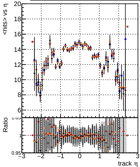
mean hit Legend: DQM_mkFit_TToriginal (blue line), DQM_mkFit_TTNEWHMS-improved (red line), DQM_mkFit_TToriginal-106 (black line), DQM_mkFit_TTNEWHMSMS-improved (orange line)
