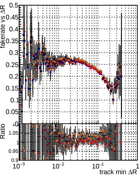
Fake rate vs \Delta R(\text{track, jet}) Legend: DOM, mktFit, TR original, DOM, mktFit, TR improved, DOM, mktFit, TR WHS-improved, DOM, mktFit, TR WHS-improved
