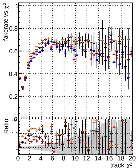
Fake rate vs. DDM mkFit TToriginal DDM mkFit TTNEWHS-improved DDM mkFit TToriginal+TTNEWHS-improved DDM mkFit TTNEWHS-improved+TTNEWHSMS-improved
