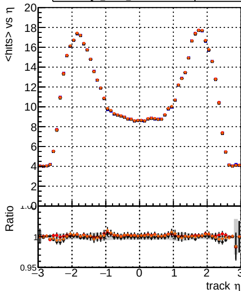
DQM_mkFit_TToriginal DQM_mkFit_TTNEWHs-improved DQM_mkFit_TToriginal-106 DQM_mkFit_TTNEWHsMS-improved mean hits
