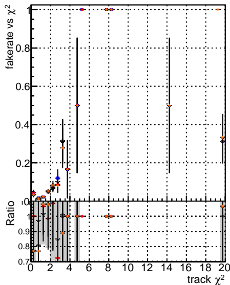
Fake rate vs. BCGM mkFit TToriginal BCGM mkFit TTWFS-improved BCGM mkFit TTWFS-improved BCGM mkFit TTWFS-improved
