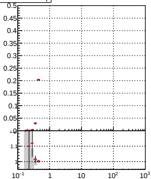
DQM_TT_mkFit_lowpT DQM_TT_mkFit_BDT_lowpT
