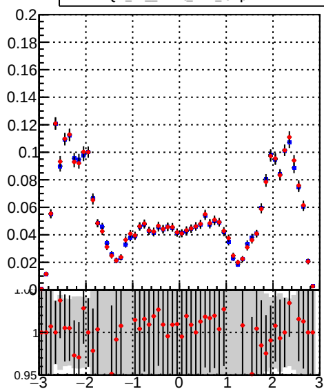
DQM_TT_mkFit_lowpT DQM_TT_mkFit_BDT_lowpT
