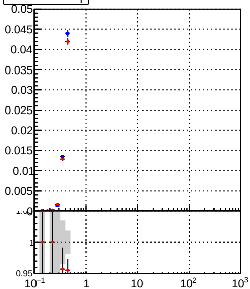
Legend: — \bullet DQM_TT_mkFit_lowpT — \bullet DQM_TT_mkFit_BDT_lowpT
