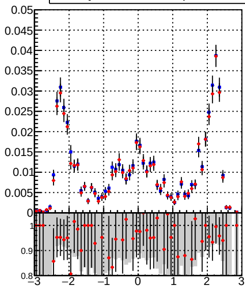
Legend: — \bullet DQM_TT_mkFit_lowpT — \bullet DQM_TT_mkFit_BDT_lowpT
