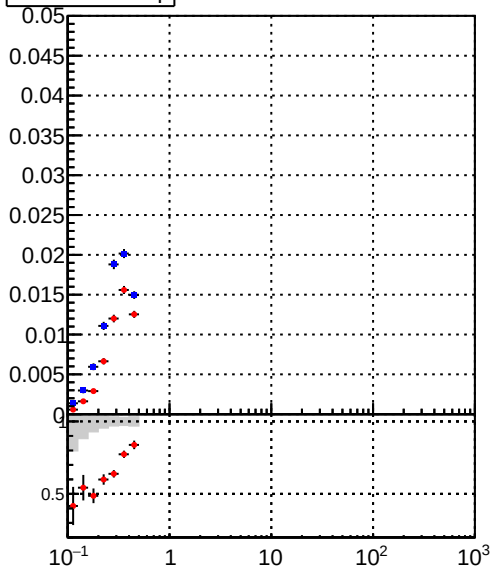
Legend: DQM_TT_mkFit_lowpT (Blue diamonds) DQM_TT_mkFit_BDT_lowpT (Red crosses)
