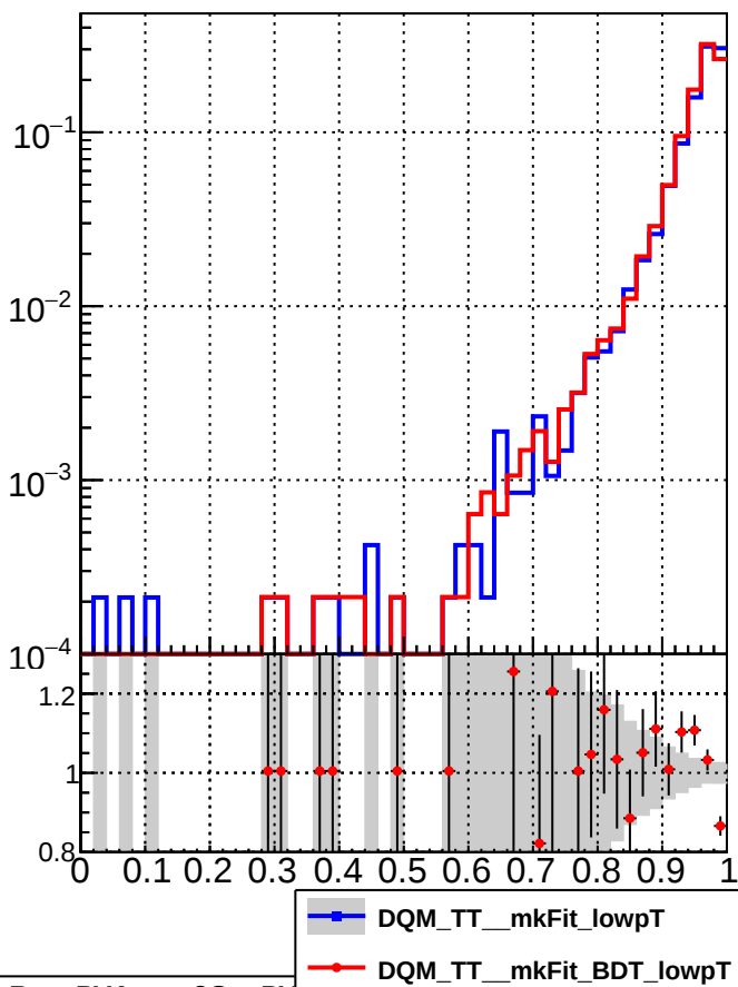
RecoPVAssoc2GenPVMatched_Missing
