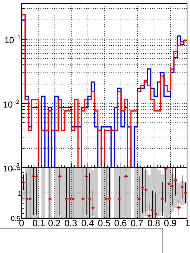
RecoPVAssoc2GenPVNotMatched_Missing
