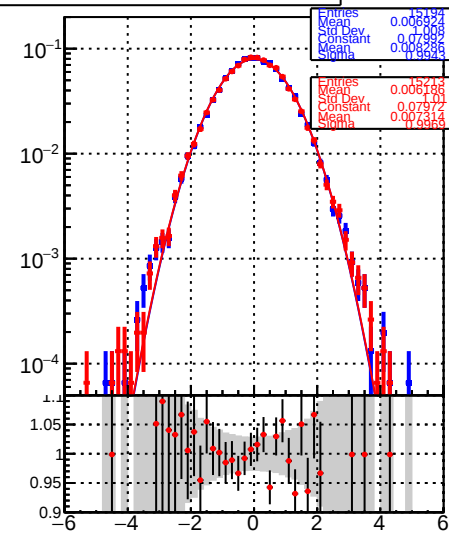
RecoAllAssoc2GenMatchedMerged_PulIZ
