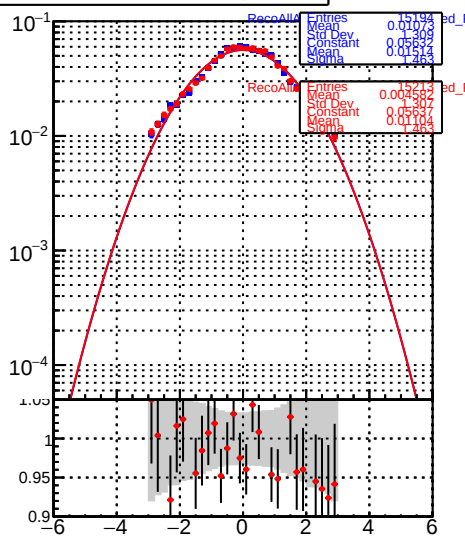
RecoAllAssoc2GenMatchedMerged_PulIZ
