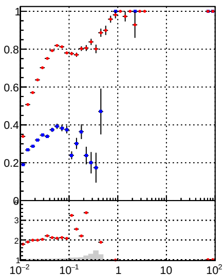
—●— DQM_TT_mkFit_lowpT —●— DQM_TT_mkFit_BDT_lowpT
