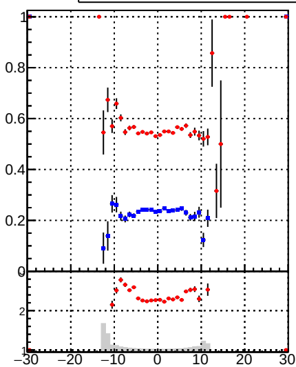
—●— DQM_TT_mkFit_lowpT —●— DQM_TT_mkFit_BDT_lowpT
