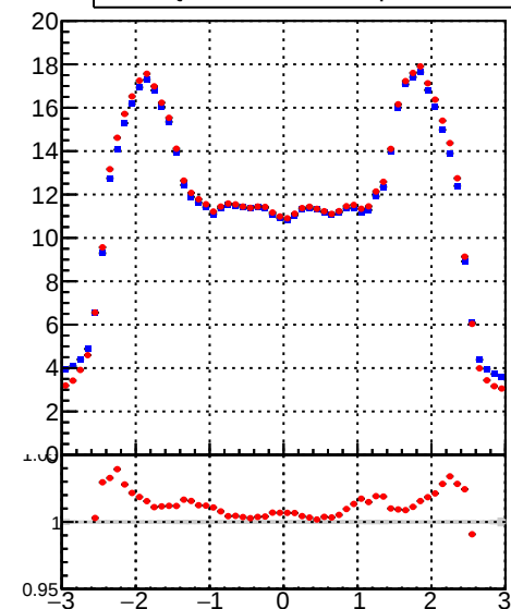
mean hit Legend: DQM_TT_mkFit_lowpT (blue line), DQM_TT_mkFit_BDT_lowpT (red line)
