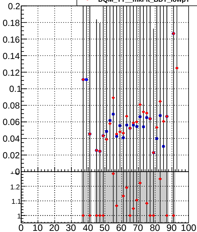
—•— DQM_TT_mkFit_lowpT —•— DQM_TT_mkFit_BDT_lowpT
