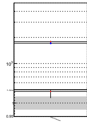
N of reco track vs. \chi^2 for DQM TT mkFit_lowT and DQM TT mkFit_BDT_lowT
