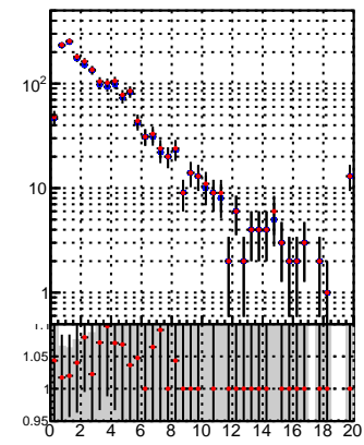
N of reco track vs. \chi^2 for DQM TT mkFit_lowT and DQM TT mkFit_BDT_lowT
