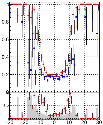
—•— DQM_TT_mkFit_lowpT —•— DQM_TT_mkFit_BDT_lowpT
