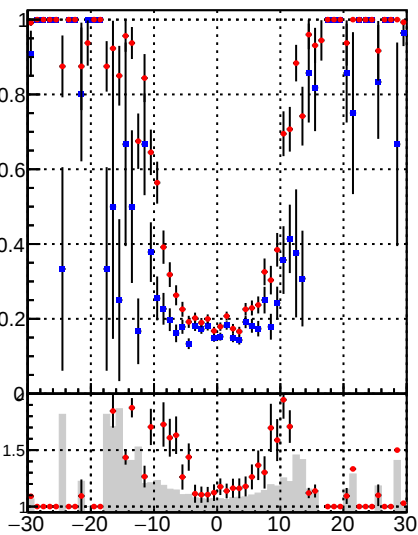
—•— DQM\_TT\_mkFit\_lowpT —•— DQM\_TT\_mkFit\_BDT\_lowpT
