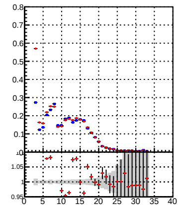
Fake rate vs hit Legend: DQM_TT_mkFit_lowpT (blue circles), DQM_TT_mkFit_BDT_lowpT (red crosses)
