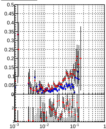
Fake rate vs \sqrt{s} — DQM_TT_mkFit_lowpT — DQM_TT_mkFit_BDT_lowpT
