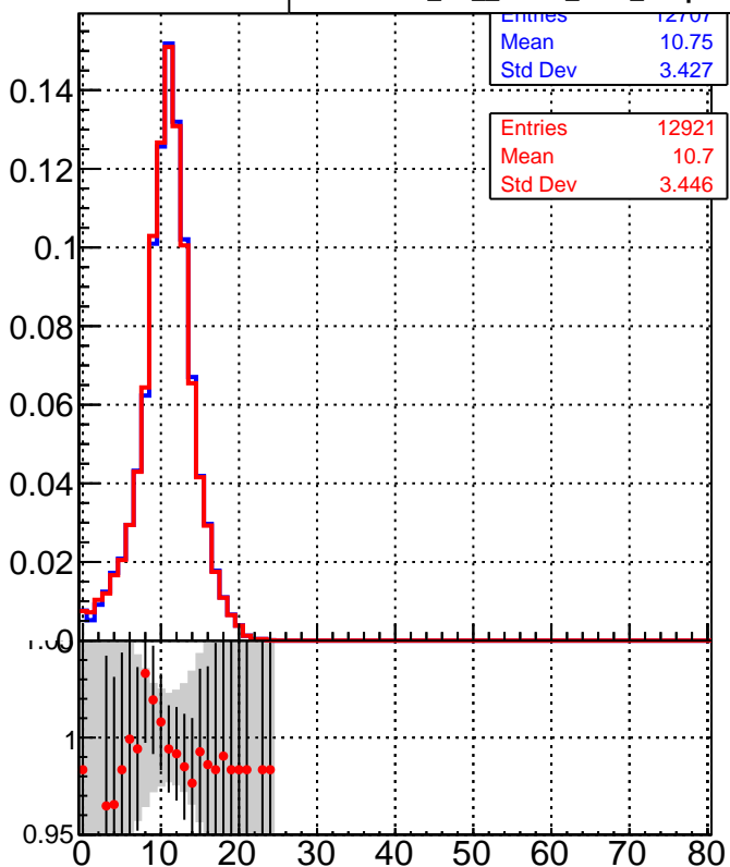
■ DQM_TT_mkFit_lowpT ● DQM_TT_mkFit_BDT_lowpT
