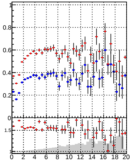
Fake rate vs. —●— DQM_TT_mkFit_lowT —+— DQM_TT_mkFit_BDT_lowT
