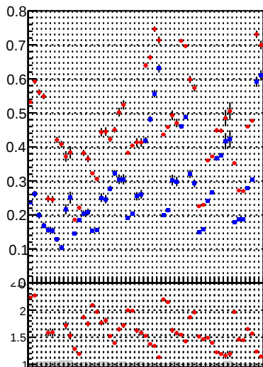
Fake rate vs. —●— DQM_TT_mkFit_lowT —+— DQM_TT_mkFit_BDT_lowT
