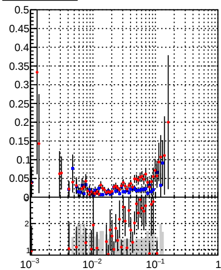
■ DQM_TT_mkFit_lowpT ● DQM_TT_mkFit_BDT_lowpT
