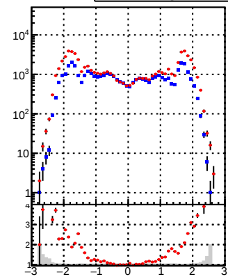
N of reco track vs \eta Legend: DQM_TT_mkFit_lowpT (blue diamonds) DQM_TT_mkFit_BDT_lowpT (red crosses)
