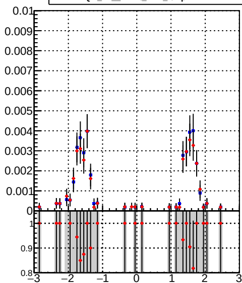
— DQM_TT_mkFit_lowpT — DQM_TT_mkFit_BDT_lowpT
