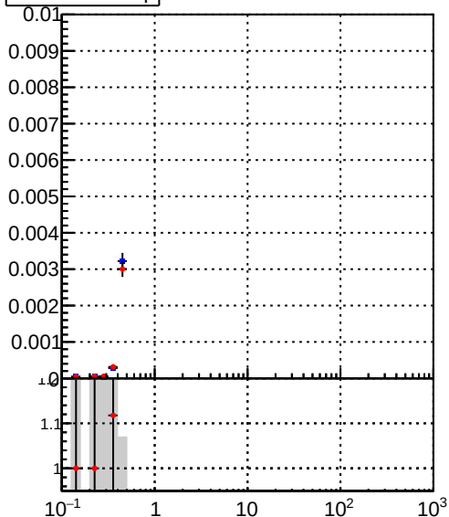
— DQM_TT_mkFit_lowpT — DQM_TT_mkFit_BDT_lowpT
