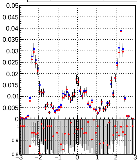
— DQM_TT_mkFit_lowpT — DQM_TT_mkFit_BDT_lowpT
