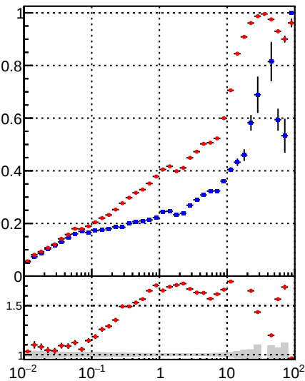
—•— DQM_TT_mkFit_lowpT —•— DQM_TT_mkFit_BDT_lowpT
