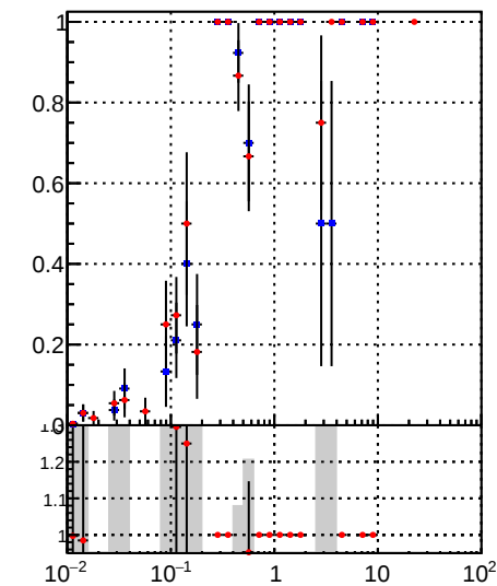
DQM_TT_mkFit_lowpT Fake rate vs v DQM_TT_mkFit_BDT_lowpT
