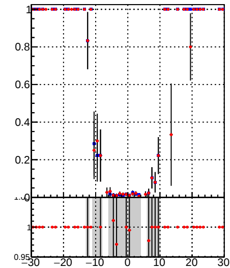
DQM_TT_mkFit_lowpT Fake rate vs v DQM_TT_mkFit_BDT_lowpT
