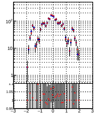
—•— DQM_TT_mkFit_lowpT —•— DQM_TT_mkFit_BDT_lowpT
