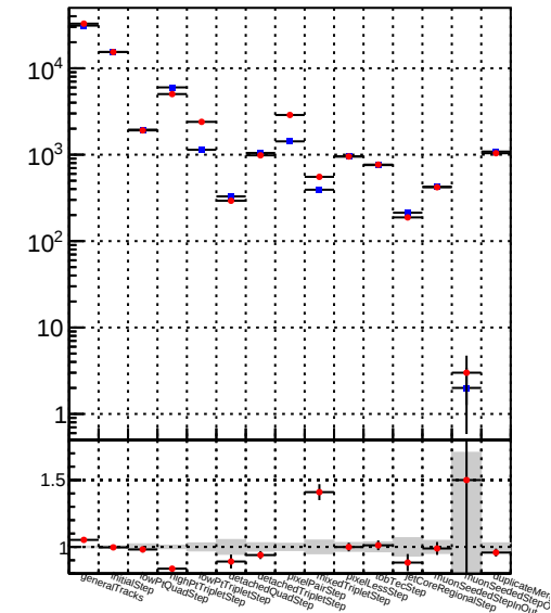
Number —●— DQM_TT__mkFit_BDT_lowpT
