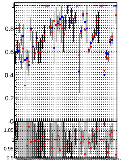
Fake rate vs. —●— DQM_TT_mkFit_lowpT —●— DQM_TT_mkFit_BDT_lowpT
