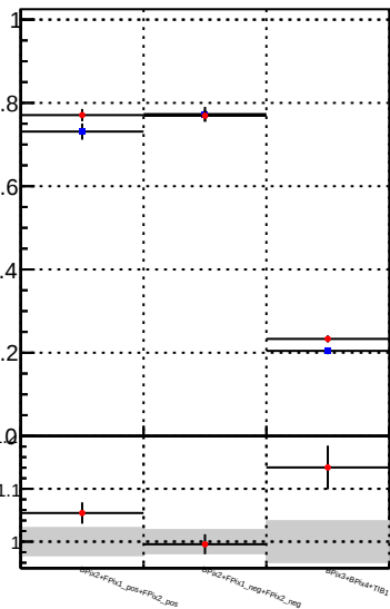
Fake rate vs. DQM_TT_mkFit_lowpT DQM_TT_mkFit_BDT_lowpT
