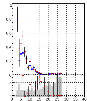
Fake rate vs hit Legend: DQM_TT_mkFit_lowpT (blue line with dots), DQM_TT_mkFit_BDT_lowpT (red line with dots)
