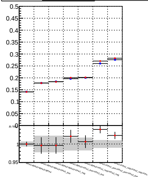
Fake rate vs. —●— DQM TT mkFit_lowT —●— DQM TT mkFit_BDT_lowT
