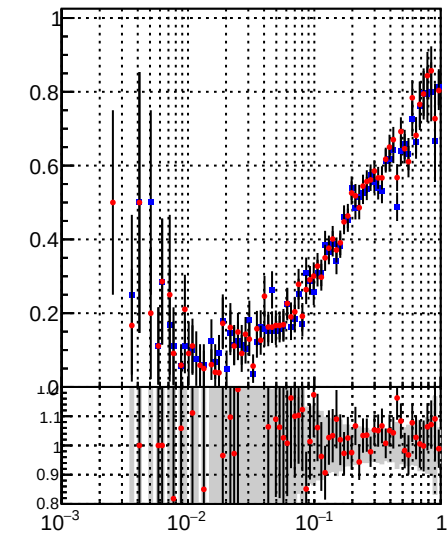
Fake rate vs \sqrt{s} DQM_TT_mkFit_lowpT DQM_TT_mkFit_BDT_lowpT
