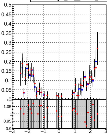
■ DQM_TT_mkFit_lowpT ● DQM_TT_mkFit_BDT_lowpT
