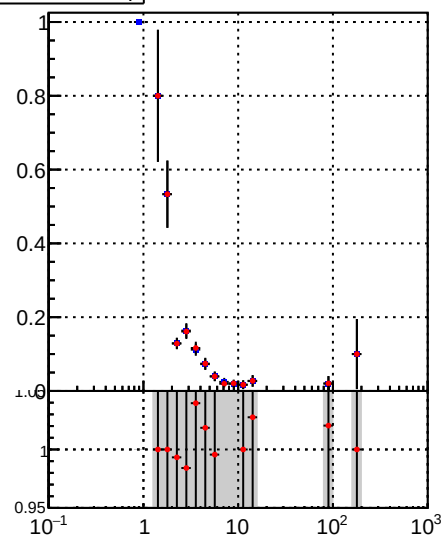
■ DQM_TT_mkFit_lowpT ● DQM_TT_mkFit_BDT_lowpT
