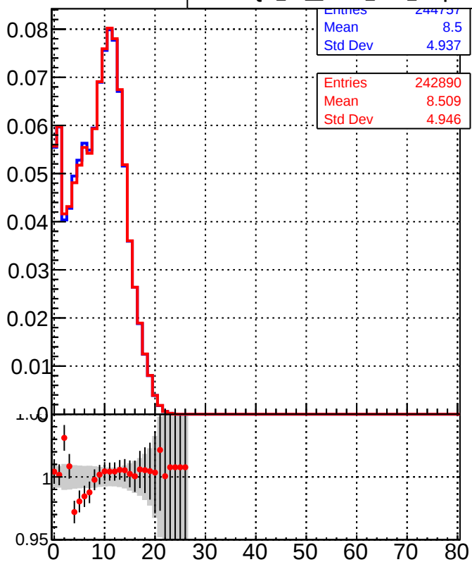
— DQM_TT_mkFit_lowpT — DQM_TT_mkFit_BDT_lowpT
