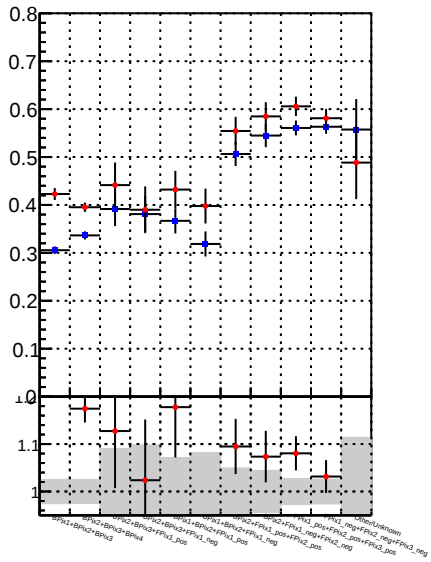
Fake rate vs. —●— DQM_TT_mkFit_lowpT —●— DQM_TT_mkFit_BDT_lowpT
