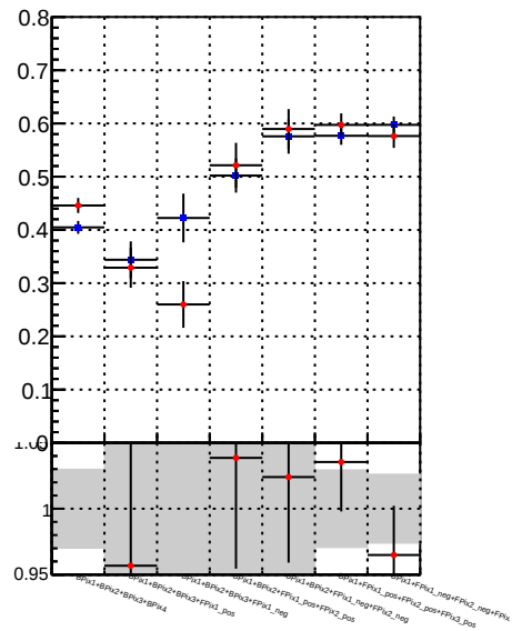
Fake rate vs. —●— DQM_TT_mkFit_lowpT —●— DQM_TT_mkFit_BDT_lowpT
