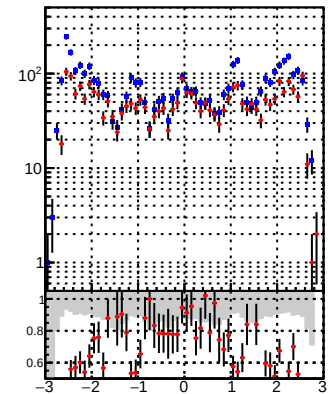
N of reco track vs \eta Legend: DQM TT mkFit lowpT (blue points) DQM TT mkFit BDT lowpT (red points)
