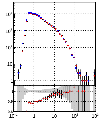
—●— DQM_TT_mkFit_lowpT —+— DQM_TT_mkFit_BDT_lowpT
