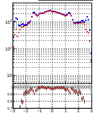
—●— DQM_TT_mkFit_lowpT —+— DQM_TT_mkFit_BDT_lowpT
