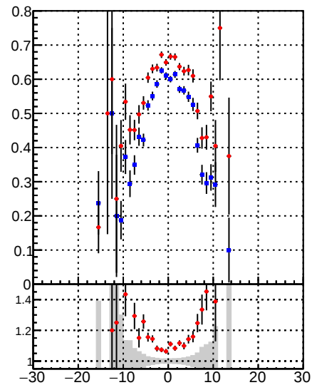
Fake rate vs d —●— DQM TT mkFit_lowpT —●— DQM TT mkFit_BDT_lowpT
