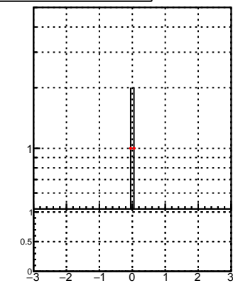
N of associated (recoToSim) duplicate tracks vs \eta —•— vs eta
