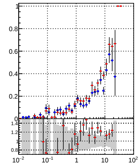
—•— DQM_TT_mkFit_lowpT —•— DQM_TT_mkFit_BDT_lowpT
