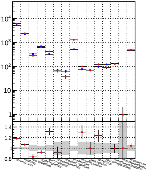
Number —●— DQM_TT_mkFit_BDT_lowpT
