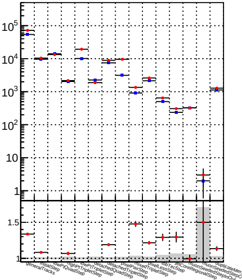
Number —●— DQM_TT_mkFit_BDT_lowpT
