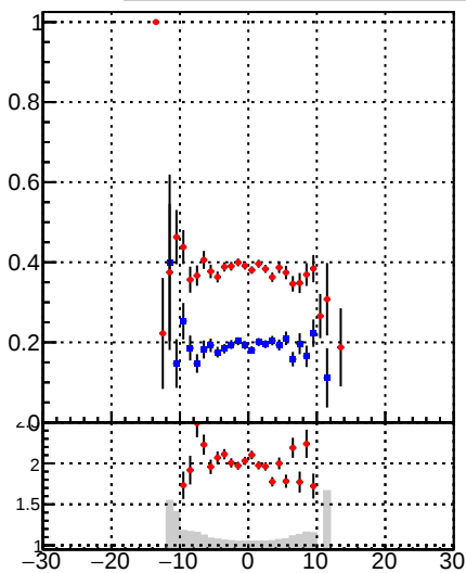
—●— DQM_TT_mkFit_lowpT —●— DQM_TT_mkFit_BDT_lowpT
